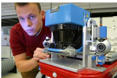
roboter kurt3d 041124 07
